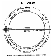
NGS Monument
